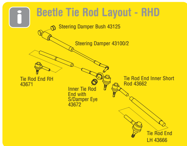
Tie Rod End with Steering Damper Eye
